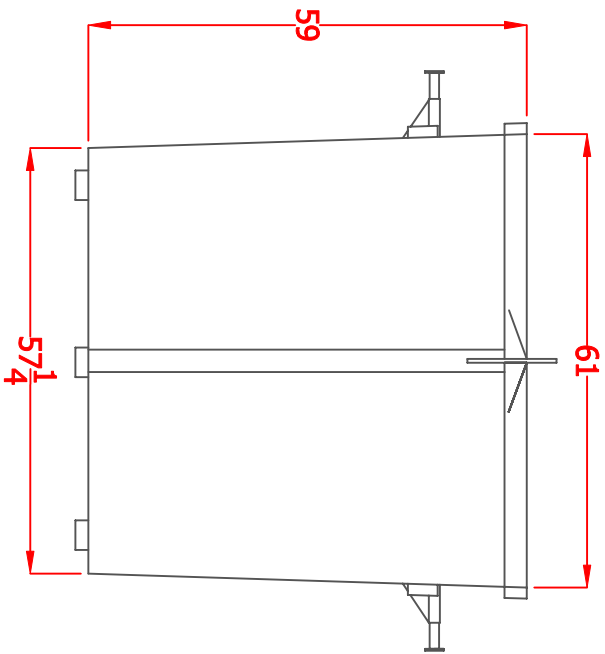
10-YARD REAR LOADER HIGH SIDE
